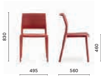
310 Polypropylene side chair
