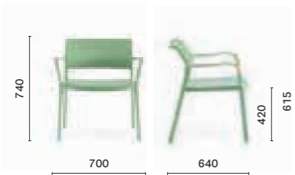
316 Polypropylene lounge armchair
