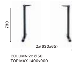
4757 Dining table base, cast-iron base
