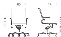
tilting support
