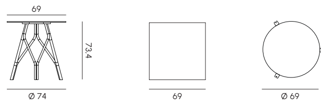
Tavolo contract 3 razze 69x69 - \varnothing 69 3 spokes contract table 69x69 - \varnothing 69
