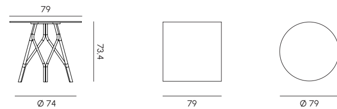
Tavolo contract 3 razze 79x79 - \varnothing 79 3 spokes contract table 79x79 - \varnothing 79
