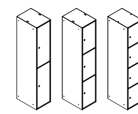
Ready Lockers L 360 P 500 H 1800 mm
