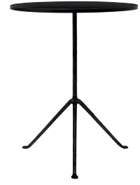
Frame: Painted Black Top: Painted Black Ø55 x H75 Ø42 x H56
