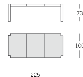
Tavolo meeting piano in legno Wooden meeting table Tables de reunion en finition bois
