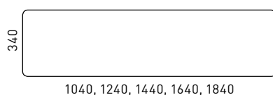
Plexiglas (Perspex) modesty panel composition
